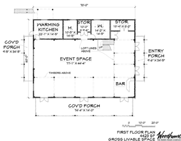
FIRST FLOOR - 4423 SQ.FT.
