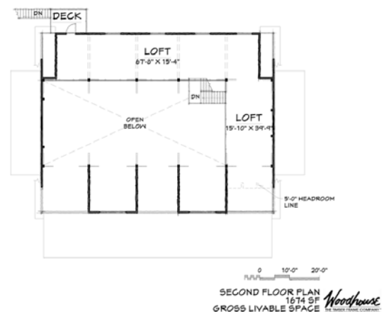
SECOND FLOOR - 1674 SQ.FT.
