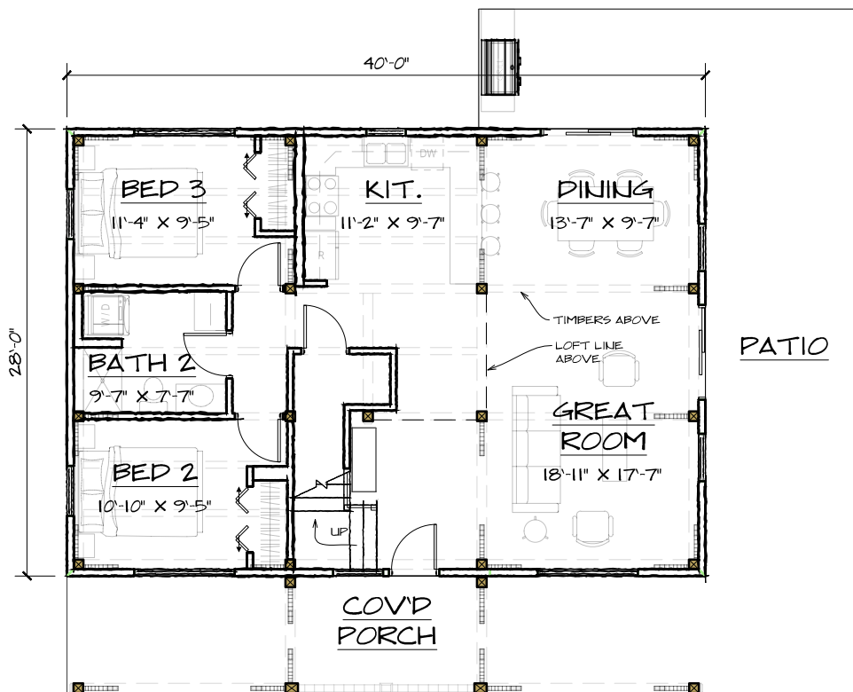
FIRST FLOOR - 1120 SQ. FT.
