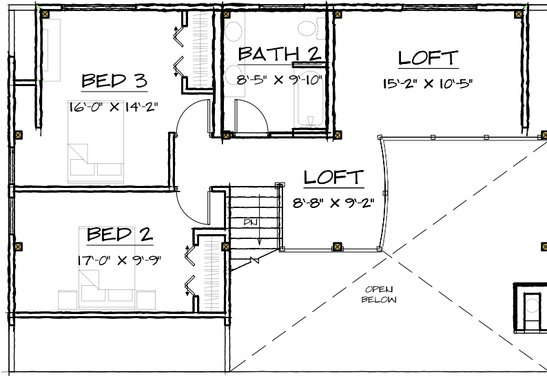
SECOND FLOOR - 800 SQ. FT.
