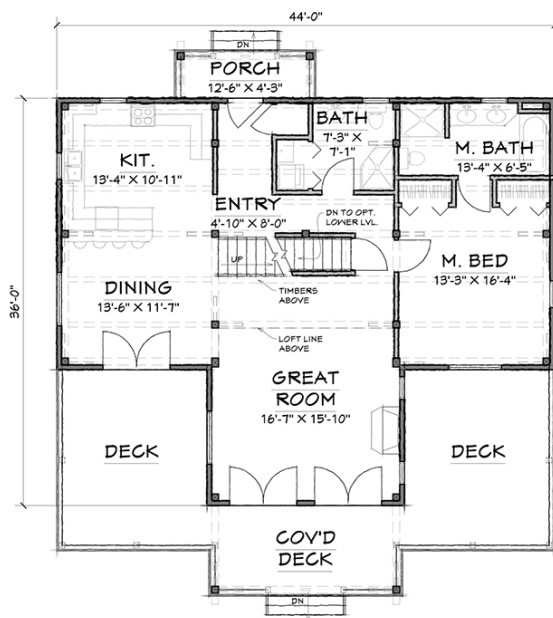
FIRST FLOOR - 1228 SQ.FT.
