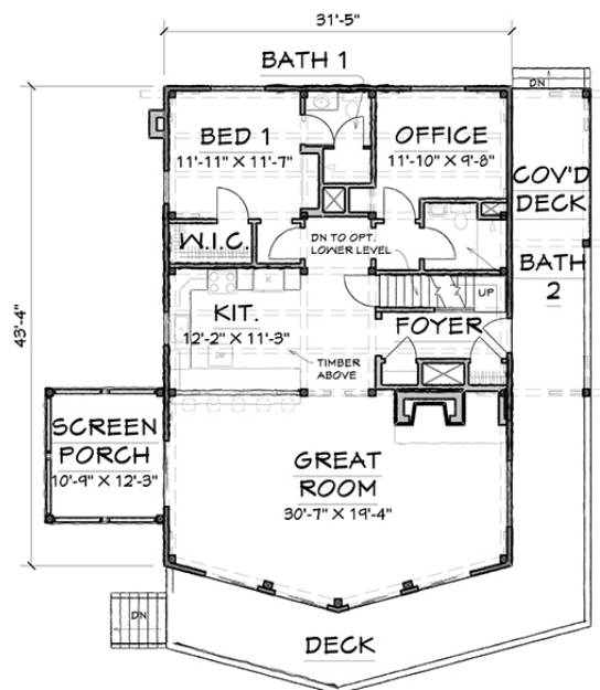
FIRST FLOOR - 1391 SQ.FT.
