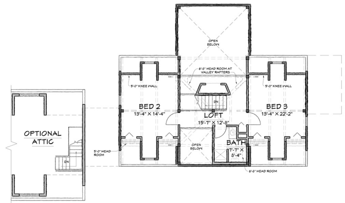
SECOND FLOOR - 749 SQ.FT.
