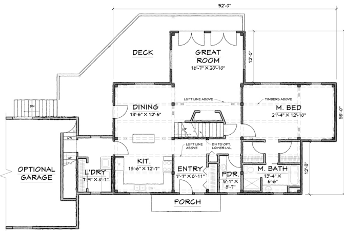
FIRST FLOOR - 1579 SQ.FT.
