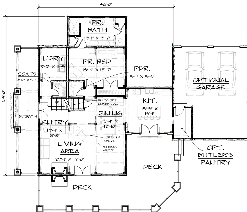
FIRST FLOOR - 1853 SQ. FT.
