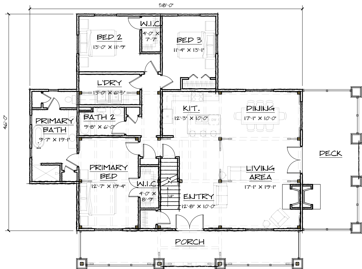
FIRST FLOOR - 2120 SQ. FT.
