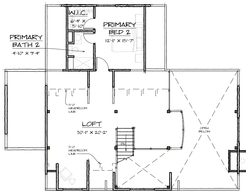
SECOND FLOOR - 938 SQ. FT.
