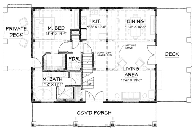
FIRST FLOOR - 1320 SQ.FT.
