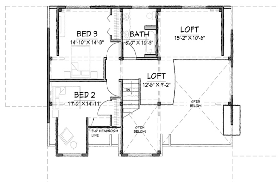
SECOND FLOOR - 802 SQ.FT.
