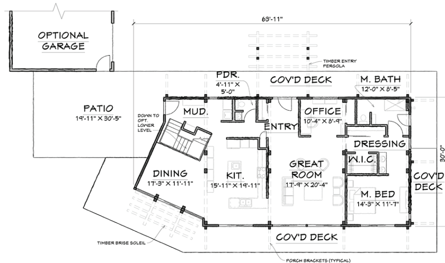
FIRST FLOOR - 1741 SQ.FT.
