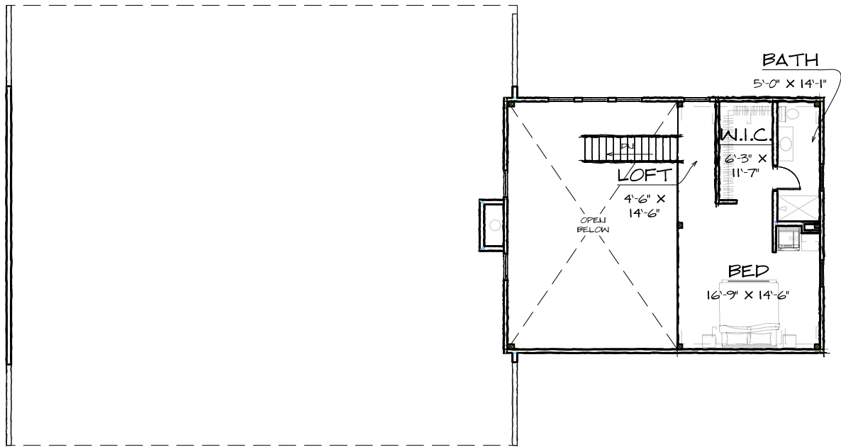
SECOND FLOOR - 513 SQ. FT.
