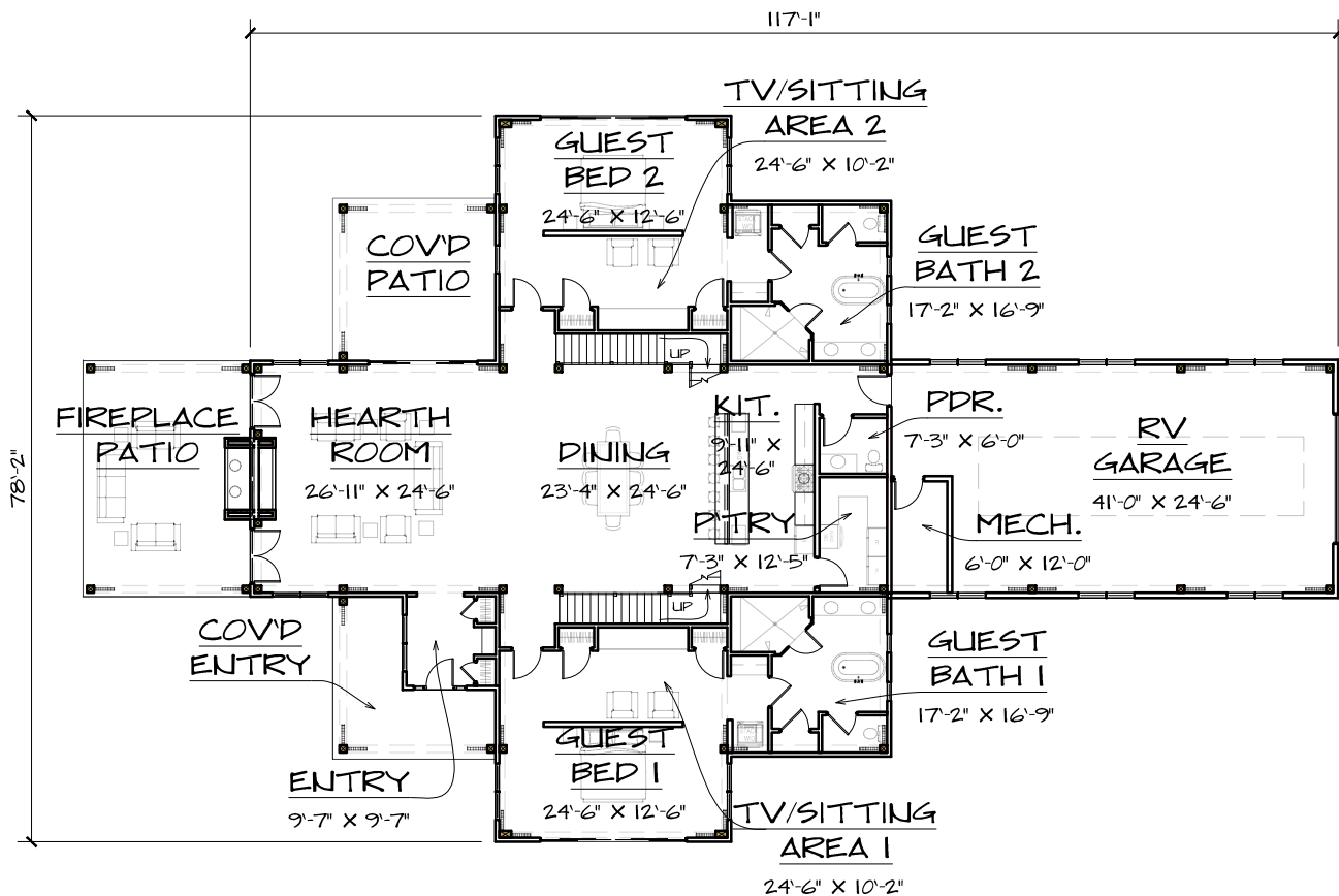
FIRST FLOOR - 3784 SQ. FT.
