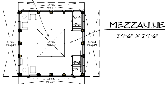
SECOND FLOOR - 473 SQ. FT.
