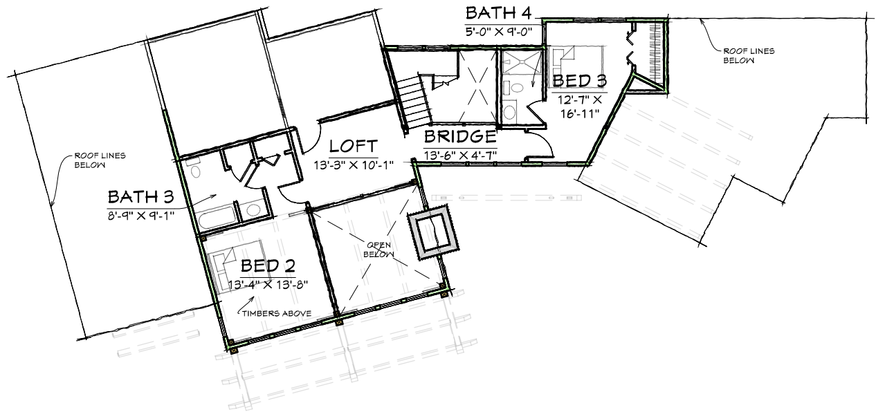
SECOND FLOOR - 813 SQ. FT.
