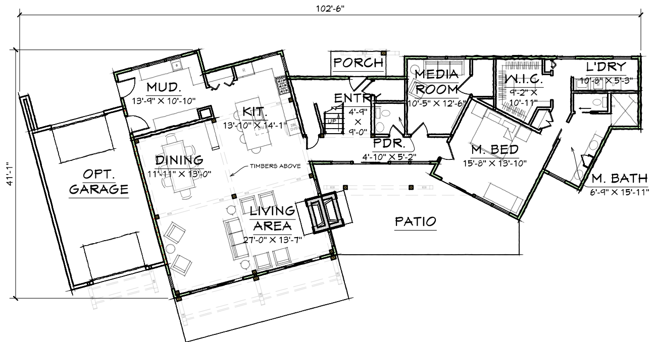
FIRST FLOOR - 2053 SQ. FT.
