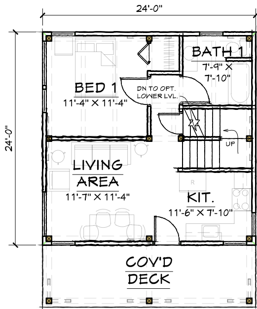
FIRST FLOOR - 524 SQ. FT.
