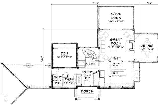
FIRST FLOOR - 1273 SQ.FT.
