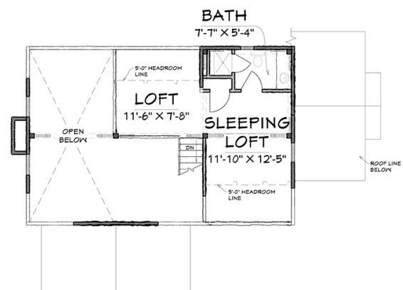
SECOND FLOOR - 367 SQ.FT.
