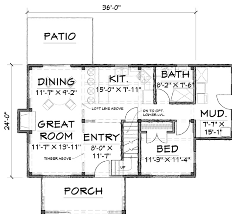
FIRST FLOOR - 947 SQ.FT.
