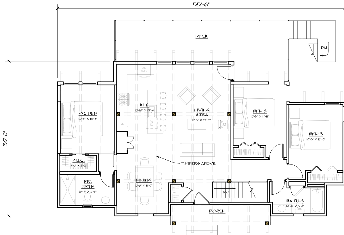
FIRST FLOOR - 1405 SQ. FT.
