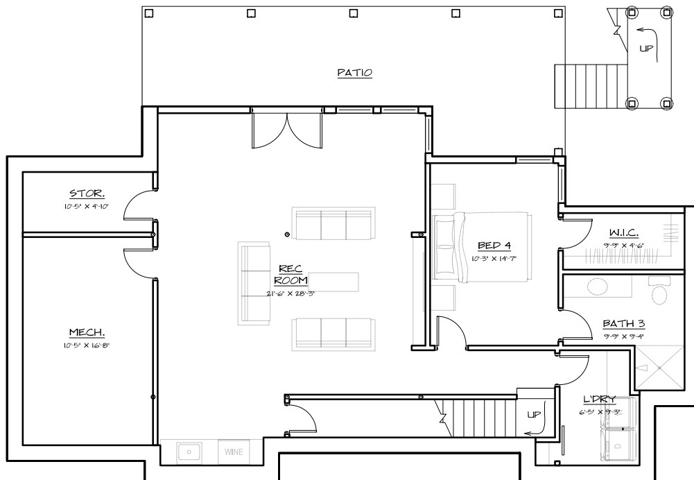
OPTIONAL LOWER LEVEL - 1017 SQ. FT.
