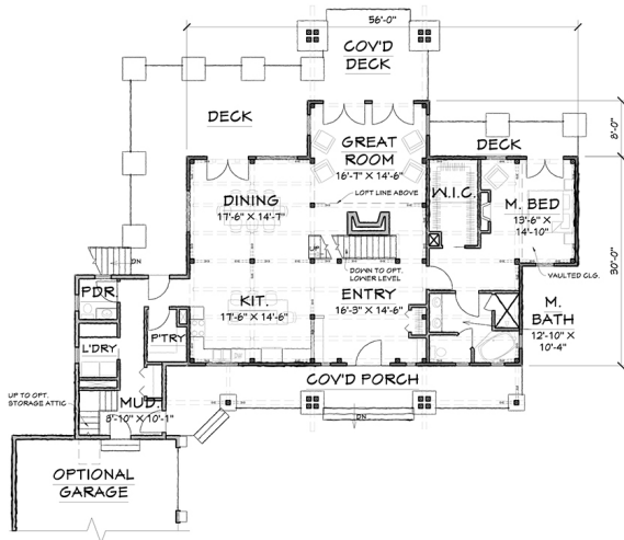
FIRST FLOOR - 2018 SQ.FT.
