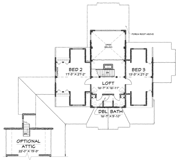
SECOND FLOOR - 1078 SQ.FT.
