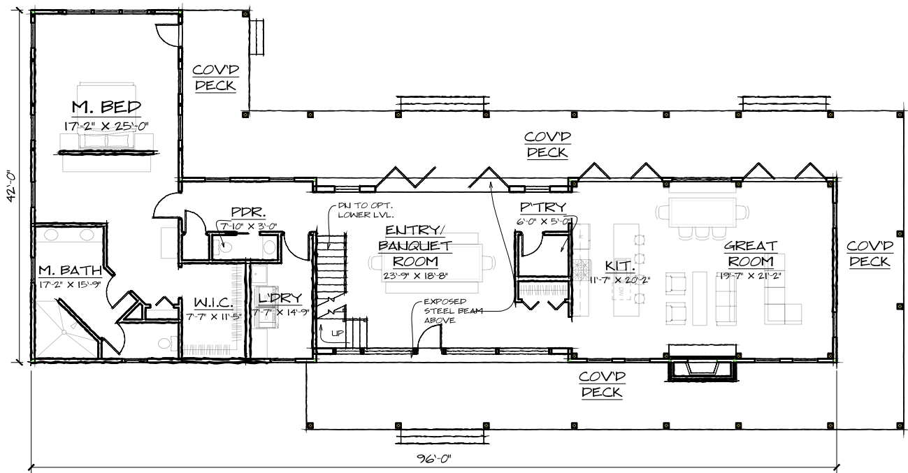
FIRST FLOOR - 2412 SQ. FT.
