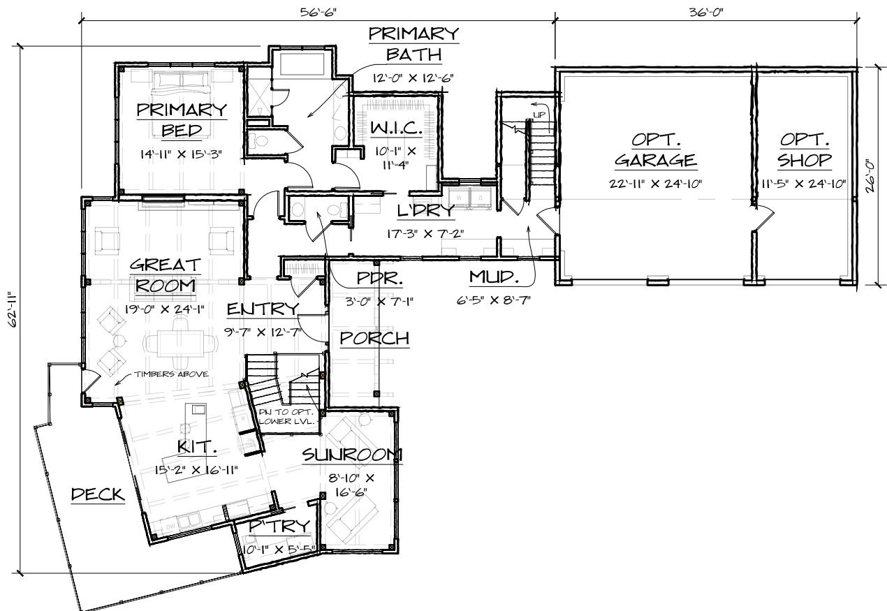
FIRST FLOOR - 2194 SQ. FT.
