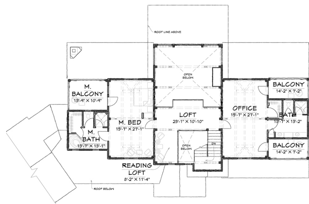
SECOND FLOOR - 1766 SQ.FT.
