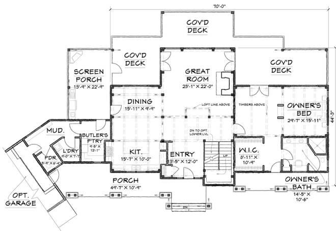
FIRST FLOOR - 2552 SQ.FT.
