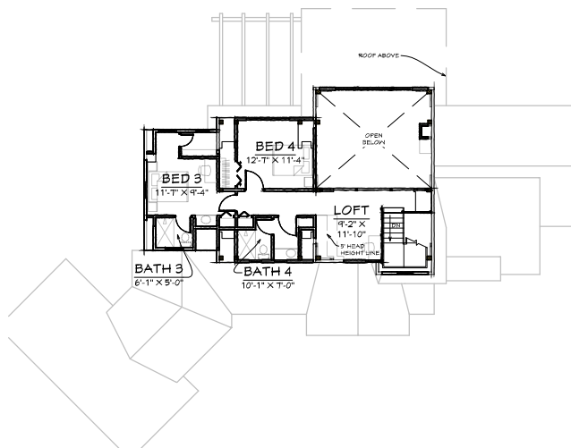
SECOND FLOOR - 713 SQ. FT.
