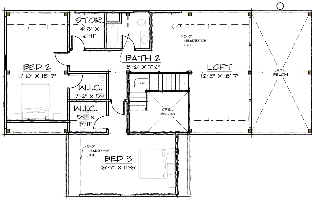
SECOND FLOOR - 1089 SQ. FT.
