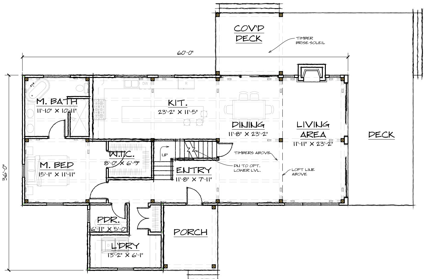
FIRST FLOOR - 1608 SQ. FT.
