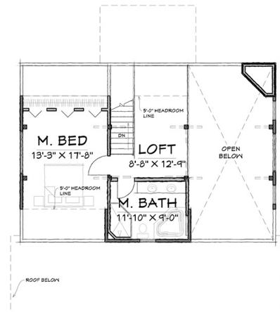
SECOND FLOOR - 503 SQ.FT.
