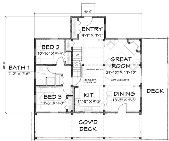
FIRST FLOOR - 1224 SQ.FT.
