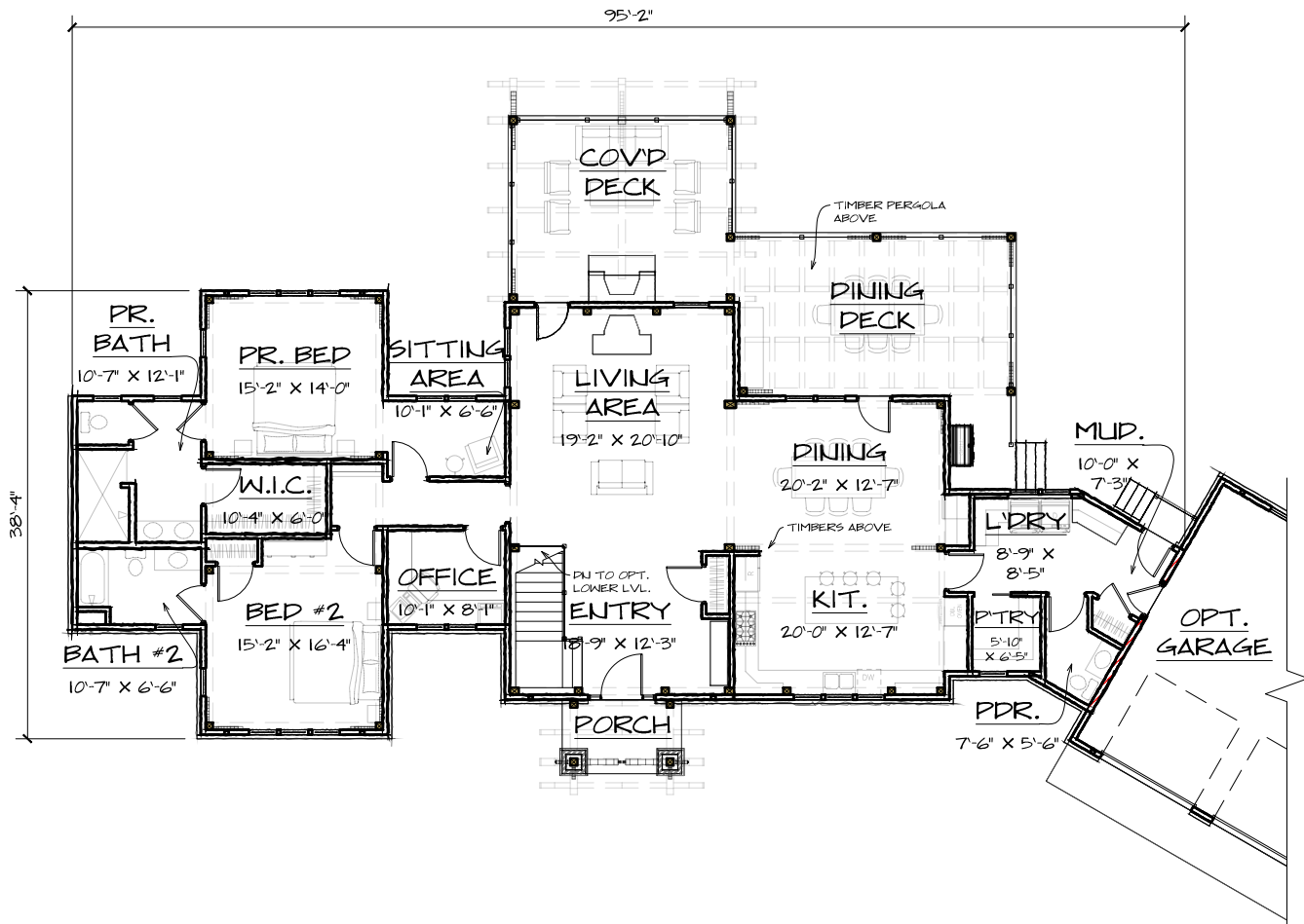
FIRST FLOOR - 2444 SQ. FT.
