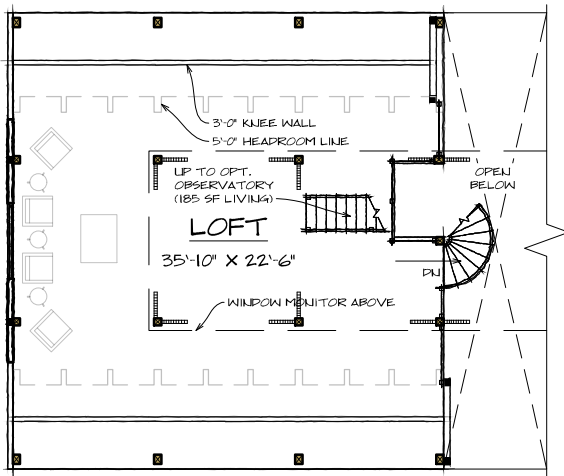
SECOND FLOOR - 912 SQ. FT.
