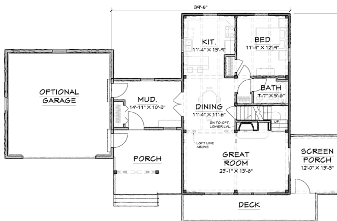
FIRST FLOOR - 1087 SQ.FT.
