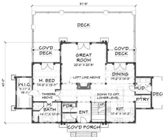
FIRST FLOOR - 2034 SQ.FT.
