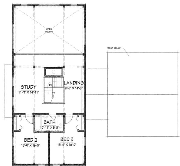
SECOND FLOOR - 1011 SQ.FT.
