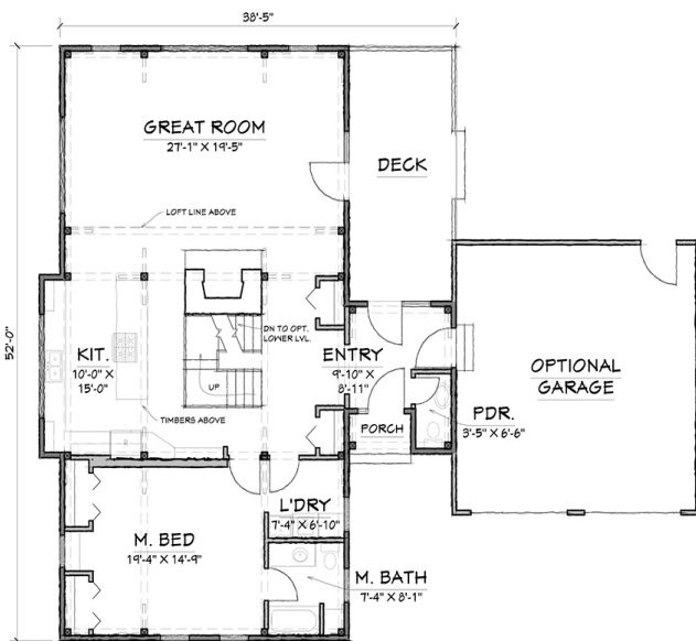
FIRST FLOOR - 1544 SQ.FT.
