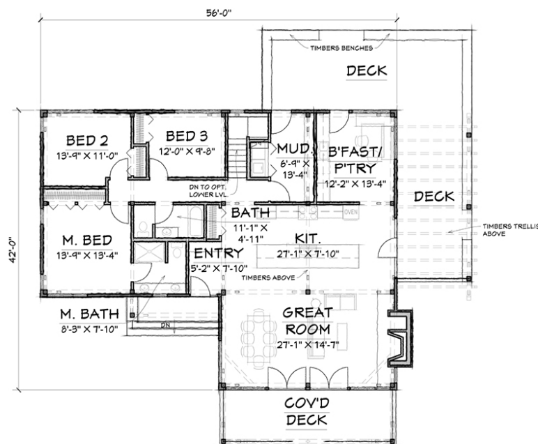
FIRST FLOOR - 1960 SQ.FT.
