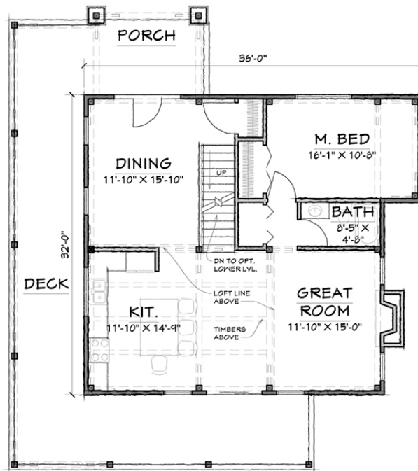
FIRST FLOOR -1028 SQ.FT.
