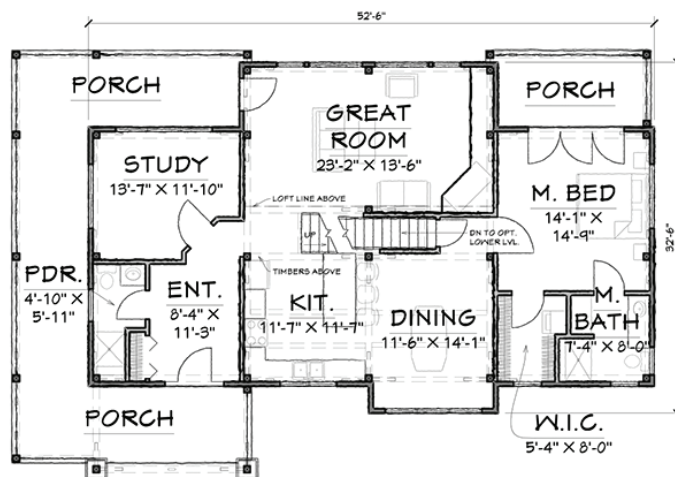
FIRST FLOOR - 1392 SQ.FT.
