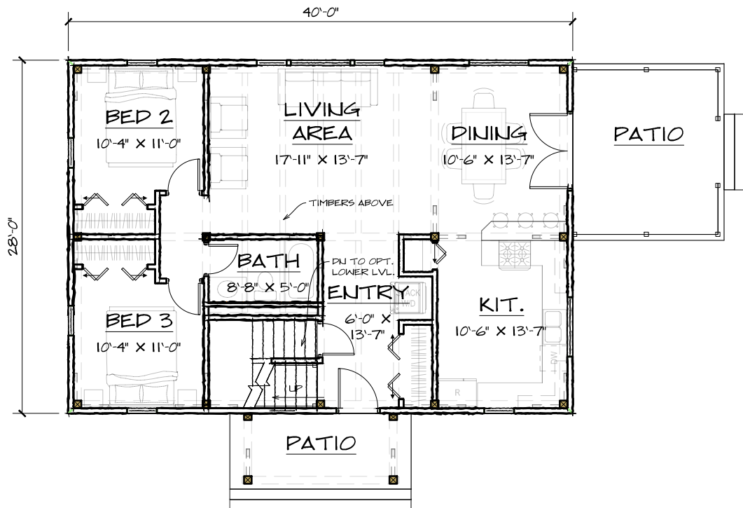
FIRST FLOOR - 1120 SQ. FT.
