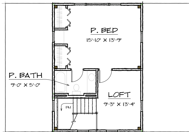
SECOND FLOOR - 477 SQ. FT.
