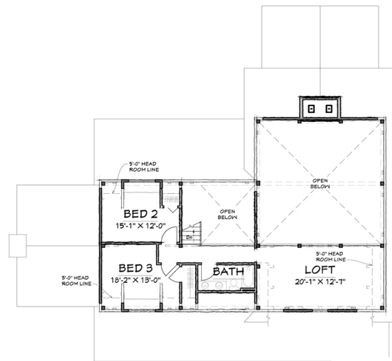
SECOND FLOOR - 772 SQ.FT.
