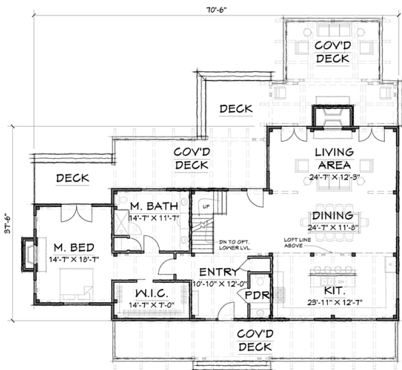
FIRST FLOOR - 2,009 SQ.FT.
