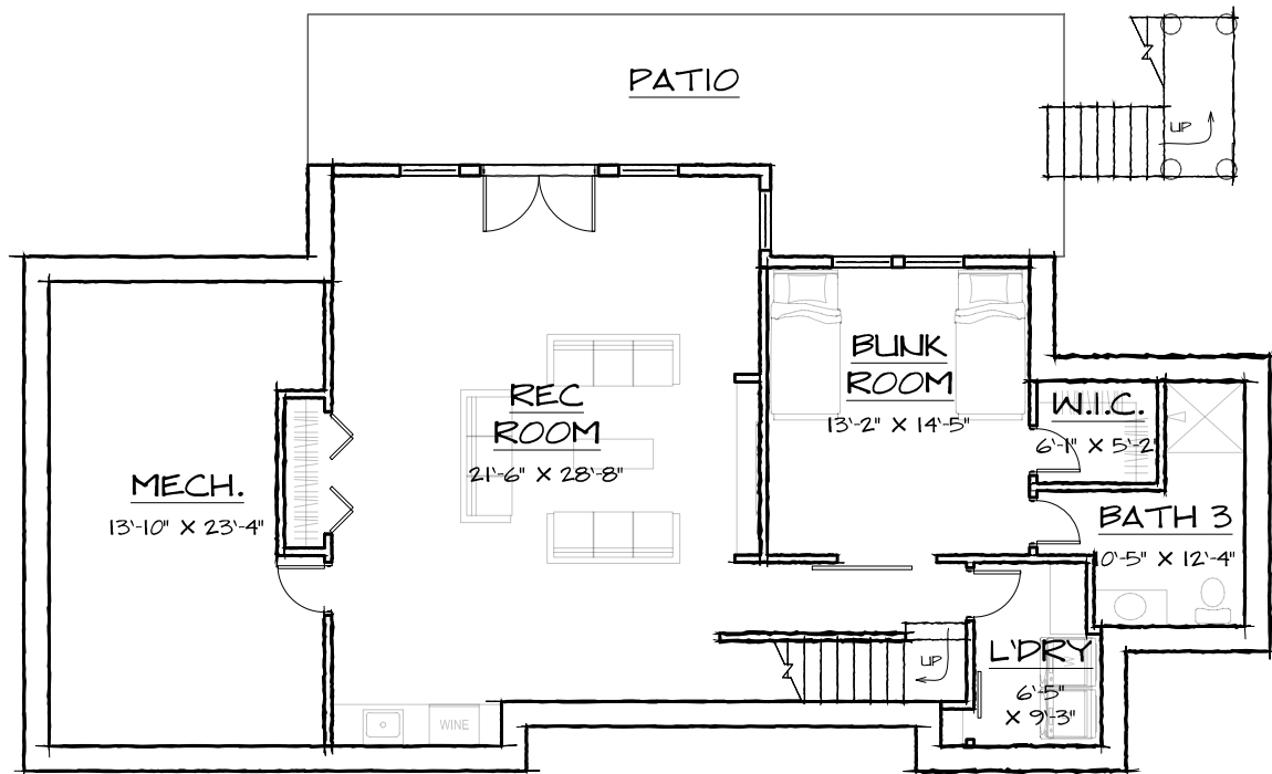
OPTIONAL LOWER LEVEL - 1083 SQ. FT.
