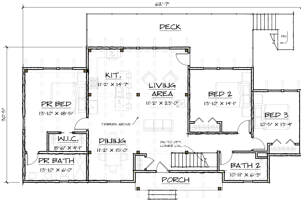
FIRST FLOOR - 1582 SQ. FT.
