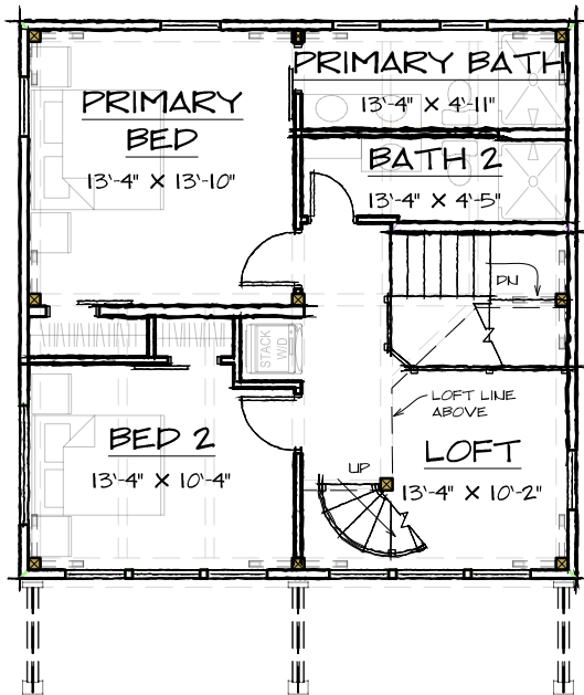
SECOND FLOOR - 721 SQ. FT.
