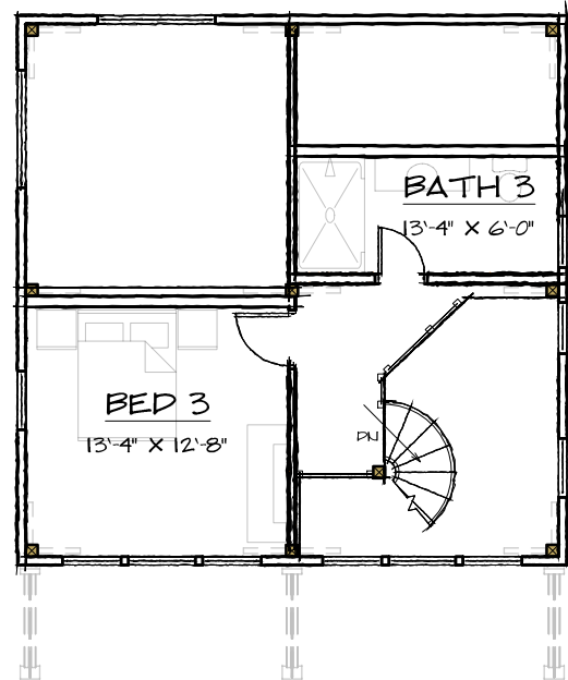
THIRD FLOOR - 361 SQ. FT.
