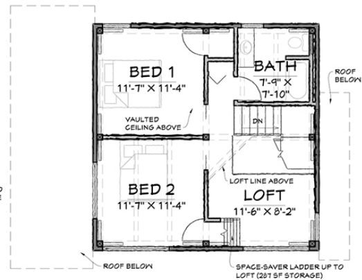
SECOND FLOOR - 517 SQ.FT.
