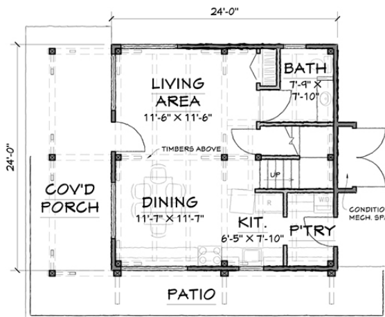
FIRST FLOOR - 576 SQ.FT.
