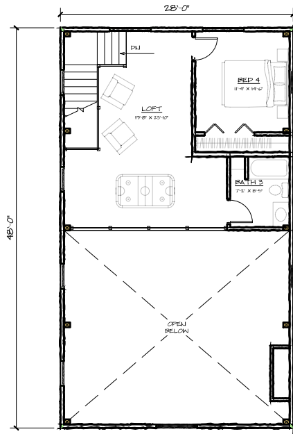
SECOND FLOOR - 601 SQ. FT.
