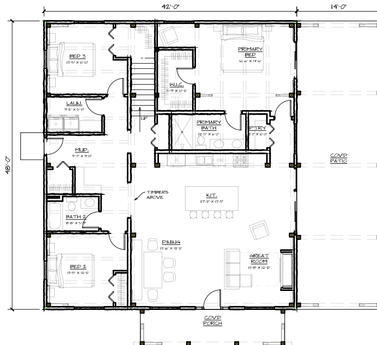
FIRST FLOOR - 2016 SQ. FT.
