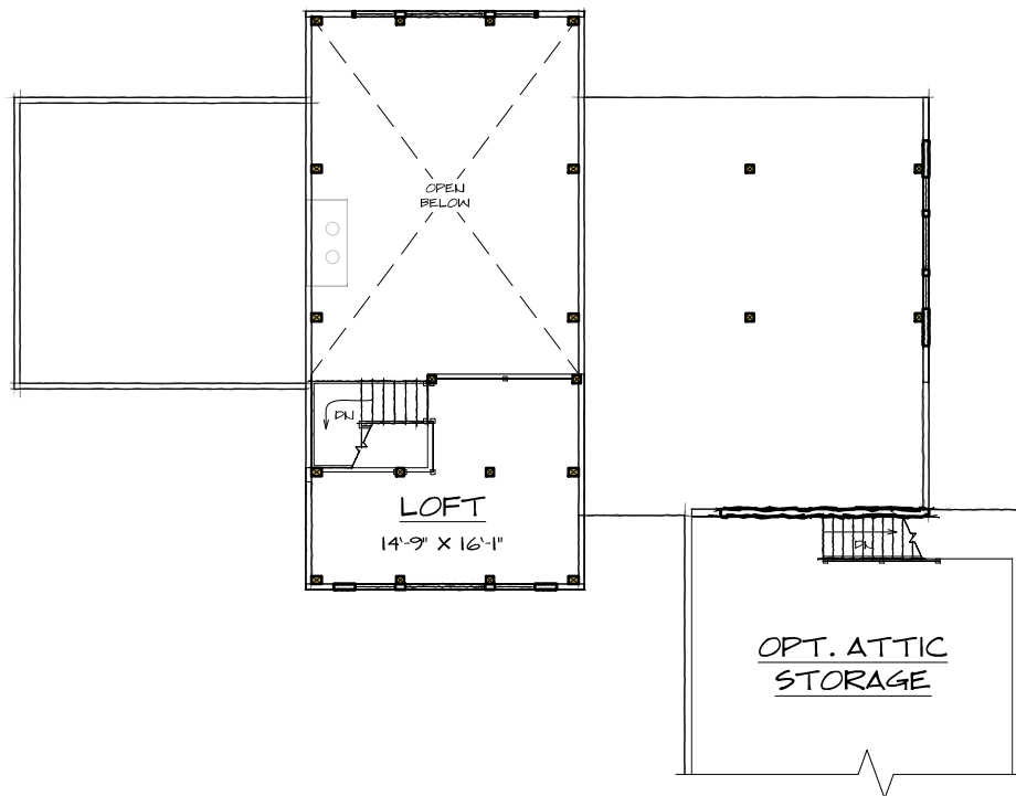
SECOND FLOOR - 198 SQ. FT.
