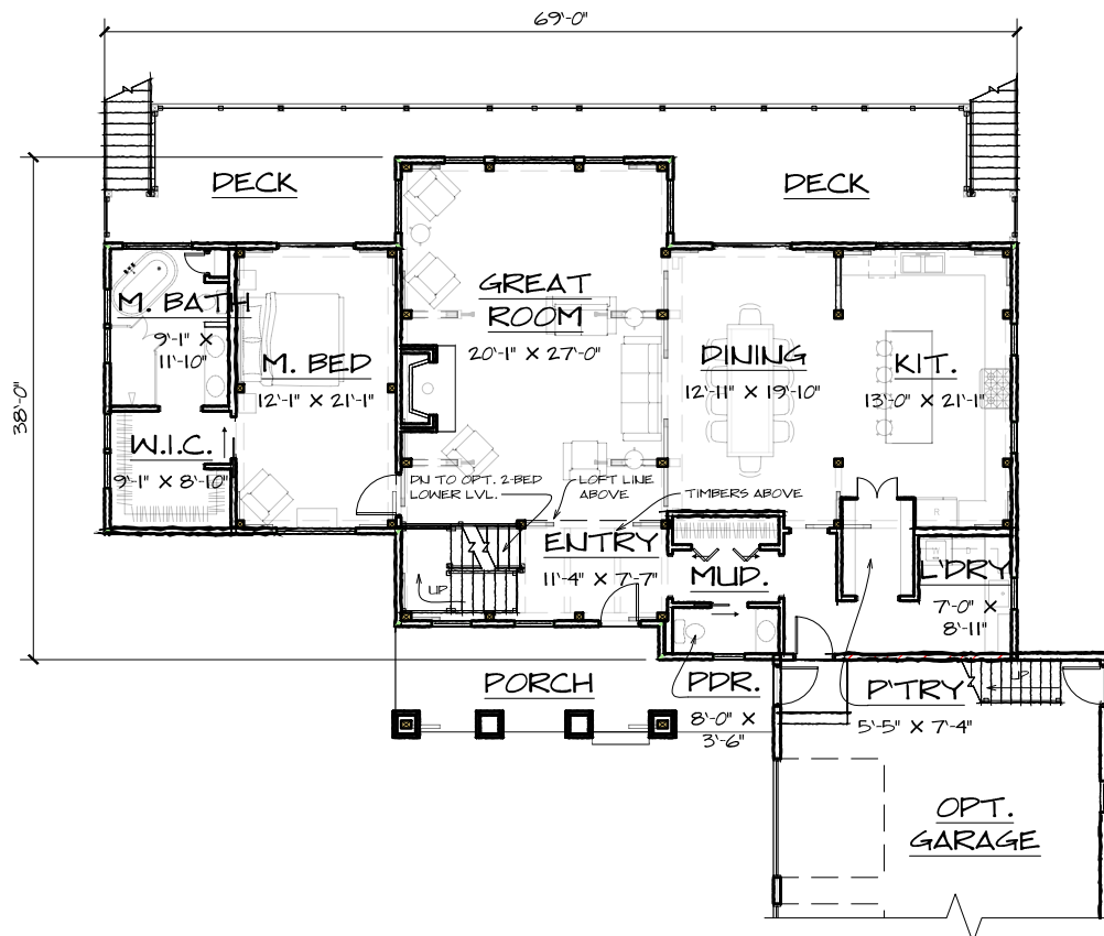
FIRST FLOOR - 2053 SQ. FT.
