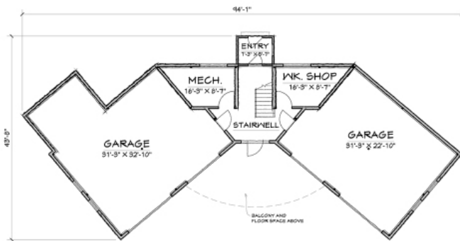
FIRST FLOOR - 2266 SQ.FT.
