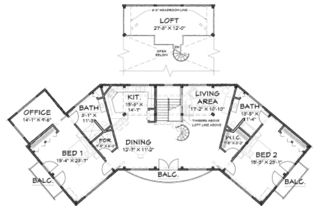
SECOND FLOOR - 303 SQ.FT.
