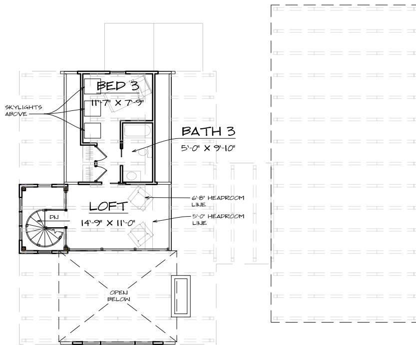
SECOND FLOOR - 383 SQ. FT.
