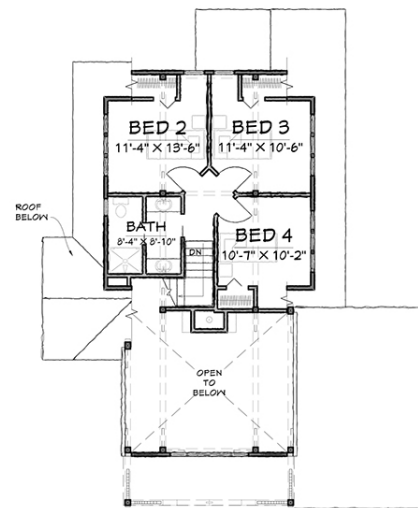
SECOND FLOOR - 623 SQ.FT.
