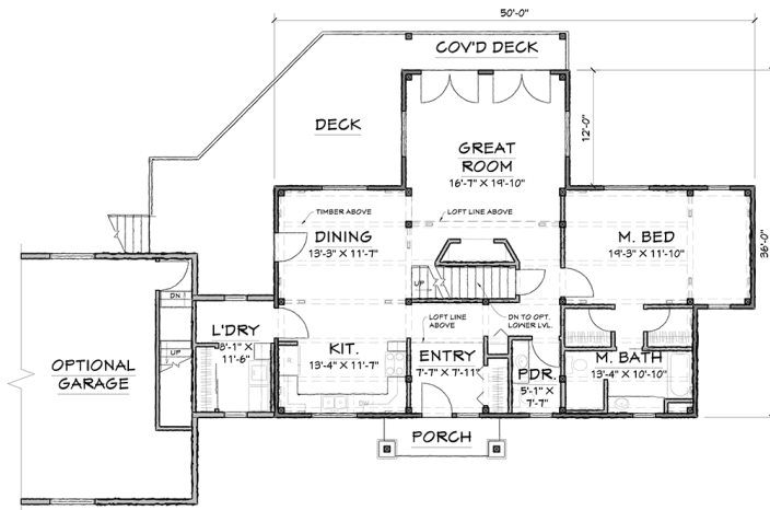
FIRST FLOOR - 1450 SQ.FT.
