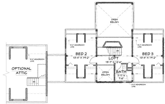
SECOND FLOOR - 710 SQ.FT.
