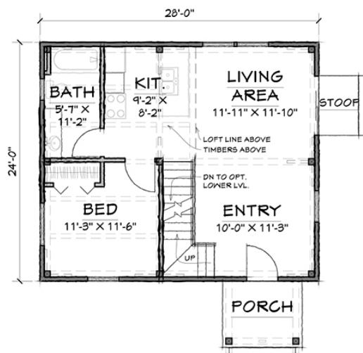
FIRST FLOOR - 630 SQ.FT.
