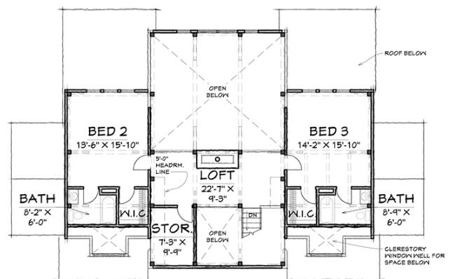
SECOND FLOOR - 894 SQ.FT.
