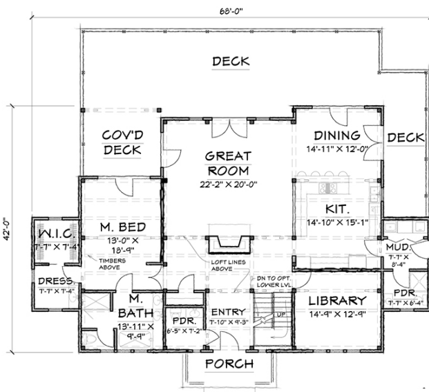
FIRST FLOOR - 2226 SQ.FT.
