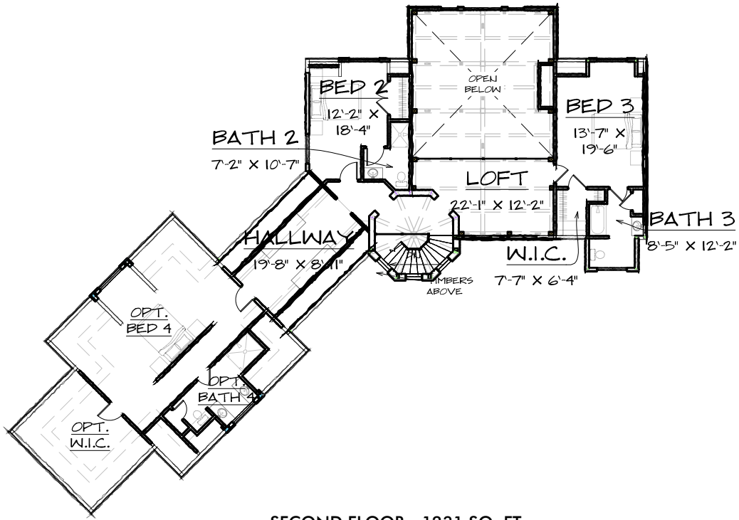
SECOND FLOOR - 1231 SQ. FT.
