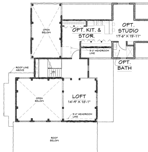
SECOND FLOOR - 950 SQ.FT.
