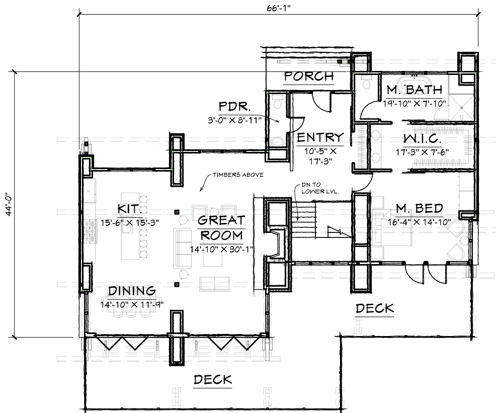
FIRST FLOOR - 1981 SQ. FT.
