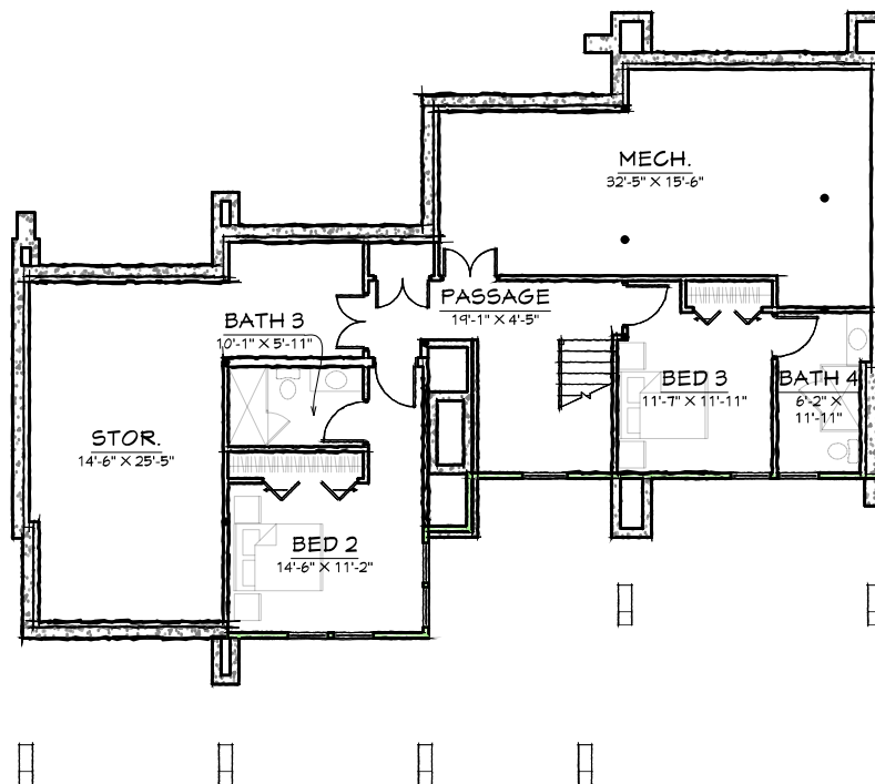
LOWER LEVEL - 738 SQ. FT.
