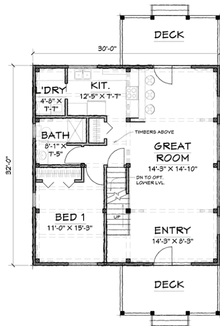
FIRST FLOOR - 925 SQ.FT.
