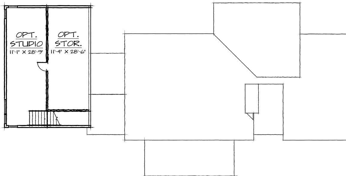
OPTIONAL SECOND FLOOR - 713 SQ. FT.
